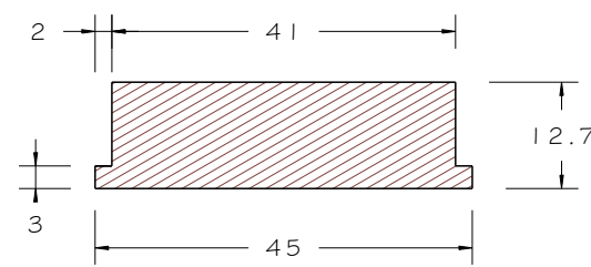
TYPICAL PLANK Scale: 1:1
