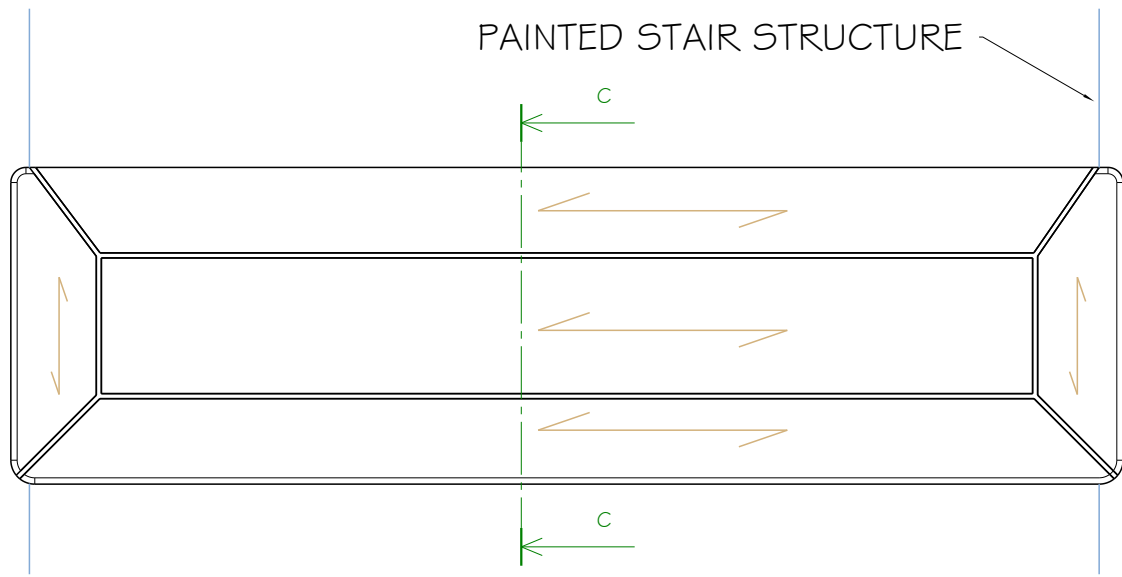
TYPICAL STEP OPEN ON BOTH ENDS Scale: 1:6
