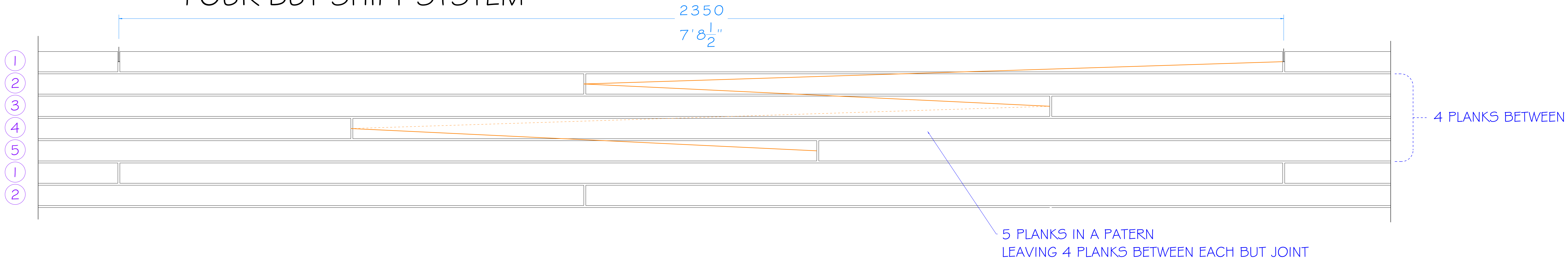
TYPICAL PLANK BUT PATTERN Scale: 1:4
