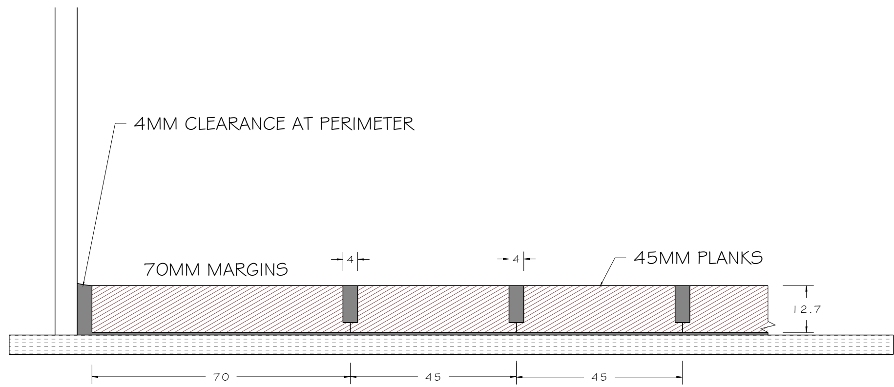
SECTION AT PLANKING Scale: 1:1
