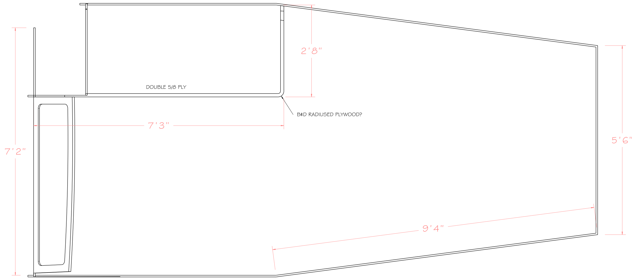
PLAN AT LOWER SKINOUT PANELS Scale: 1:16
