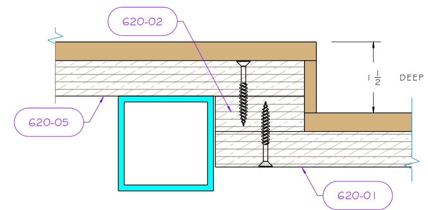
LOOKING TO PORT @ AFT END Scale: 1:2
