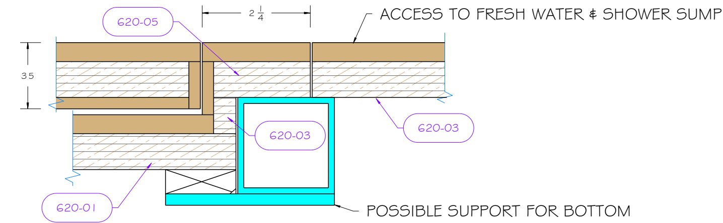
LOOKING TO PORT @ FWD END Scale: 1:2
