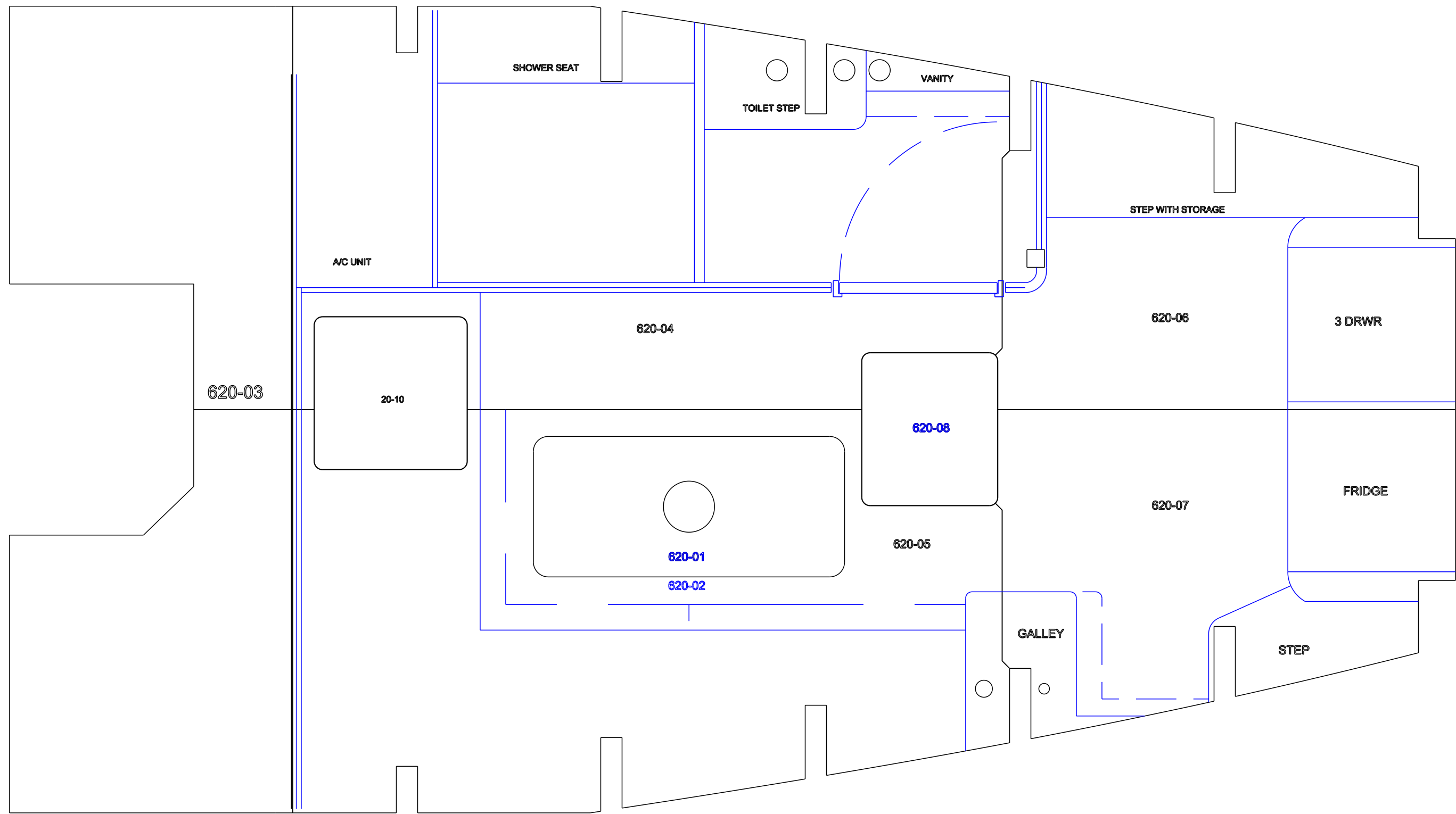
SOLE ROUGH IN PANELS Scale: 1:1/2
