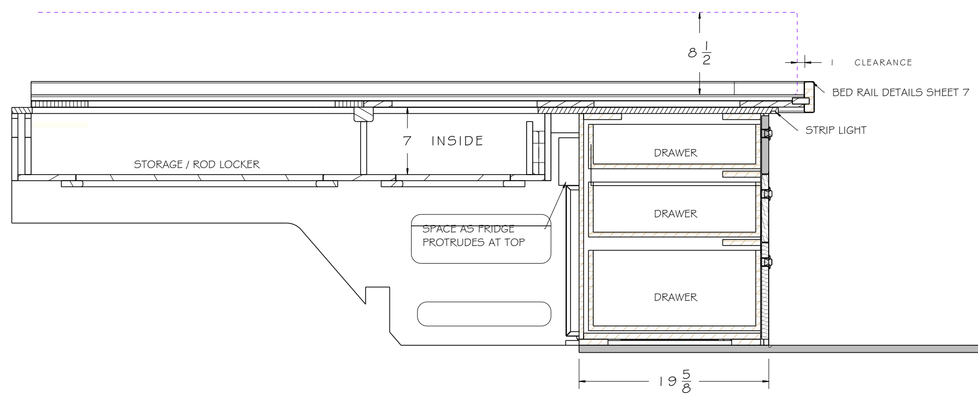
SECTION @ DRAWER UNIT Scale: 1:10
