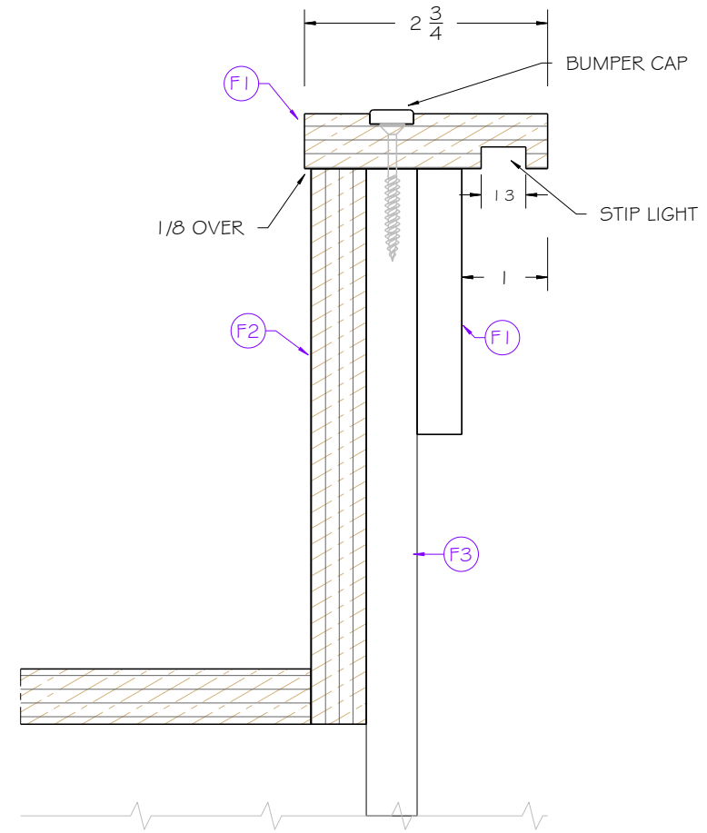
Section cut L-L Scale: 1:2
