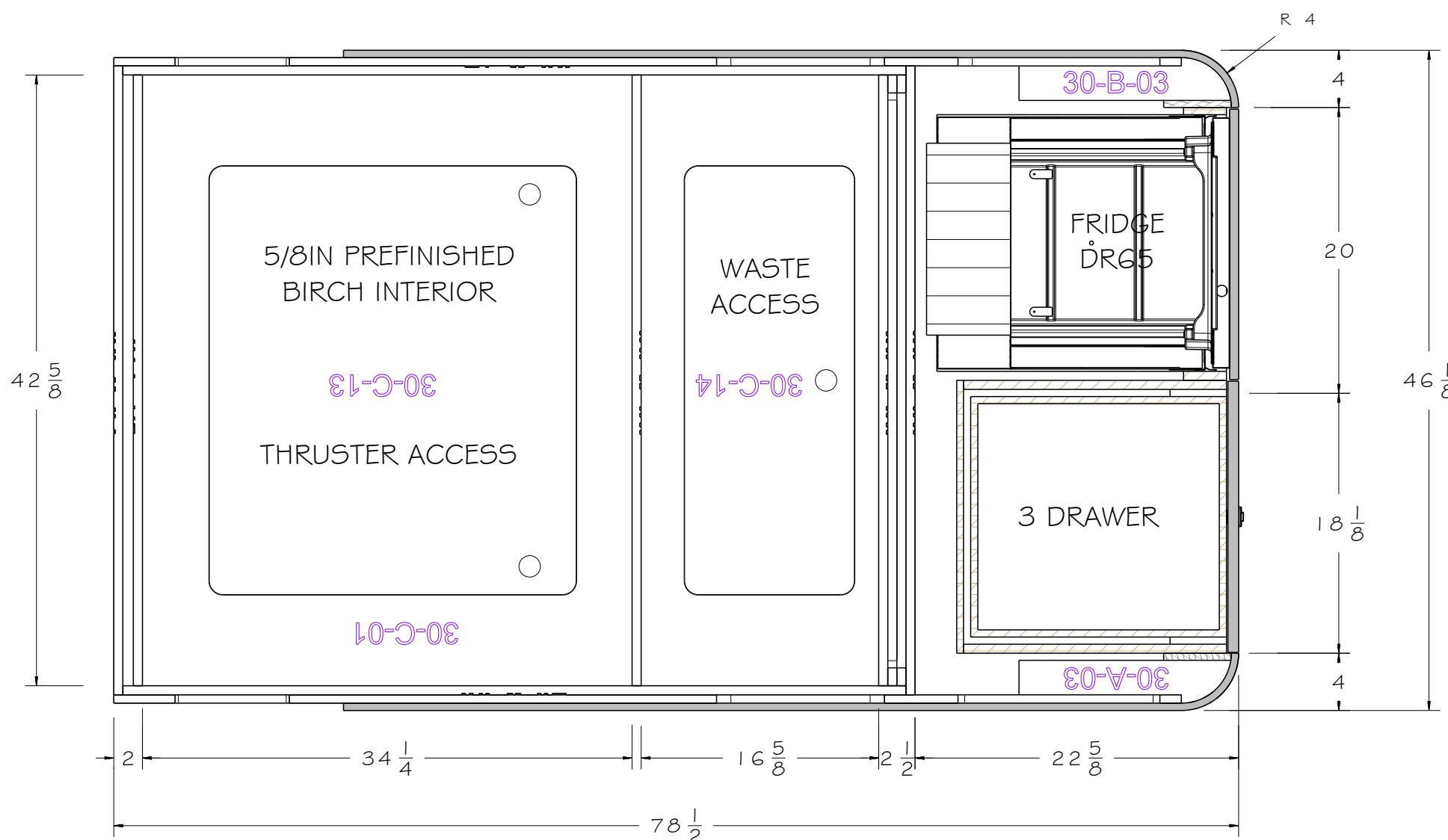
SECTION @ STORAGE UNDER MATTRESS Scale: 1:10
