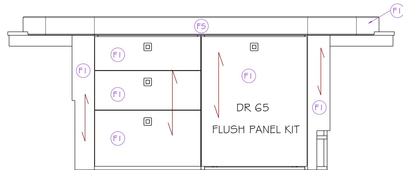
LOOKING FORWARD Scale: 1:10
