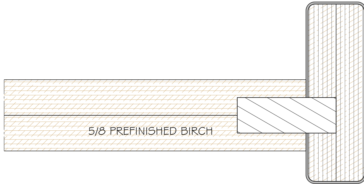
RAIL DETAIL Scale: 1:1
