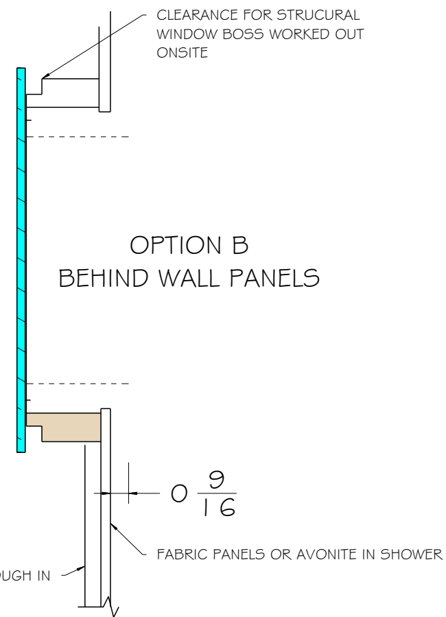
Section view A-A[2]
