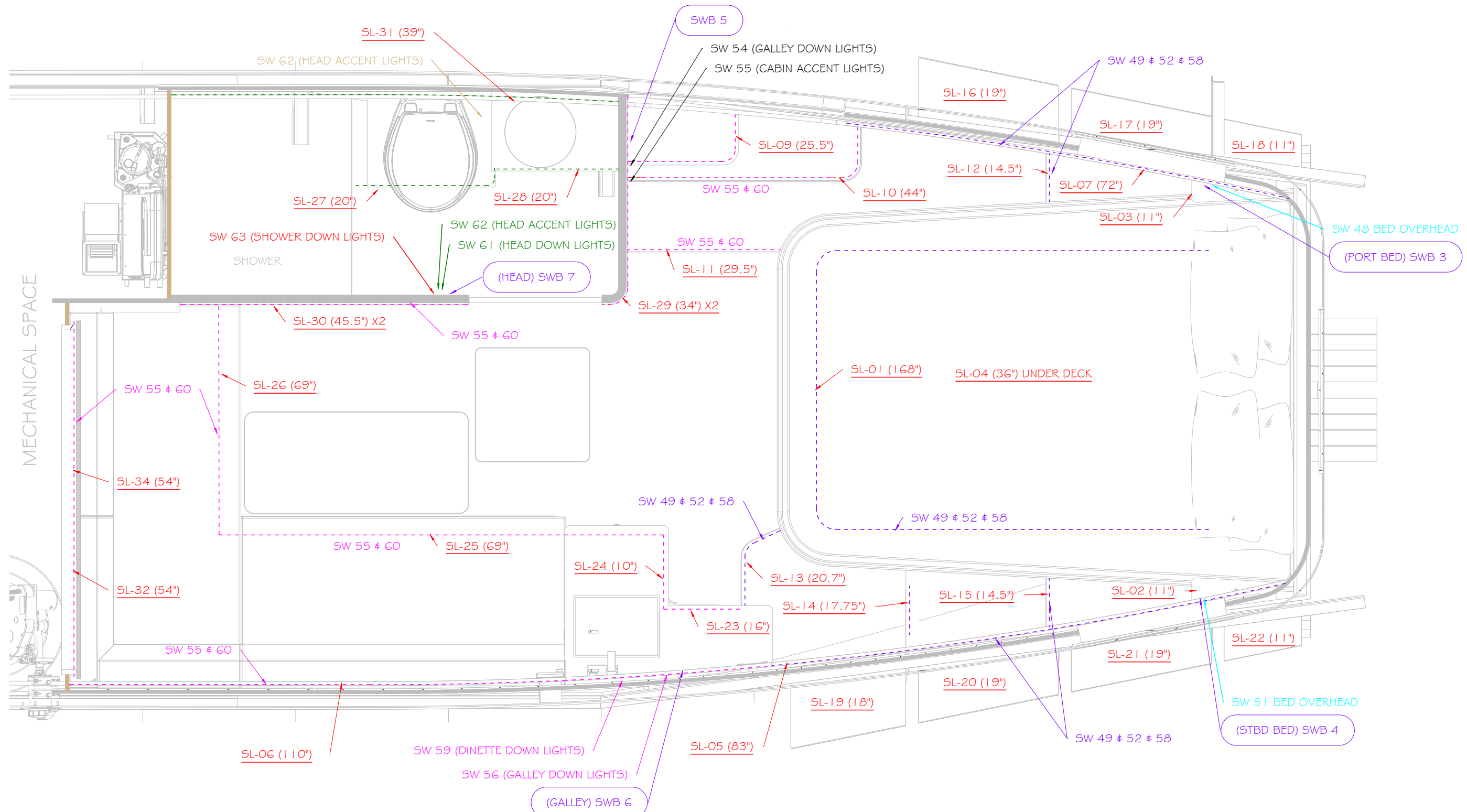
PLAN @ STATEROOM Scale: 1:16
